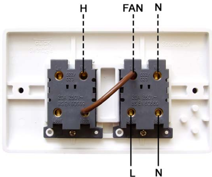
Fig 1: Connections for Heat Zone
