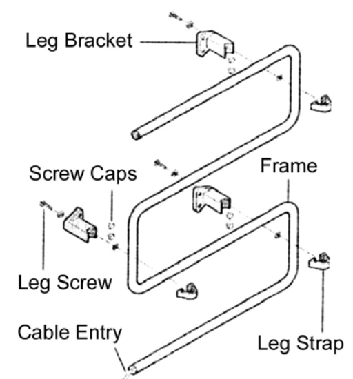
Figure 1 : TRJ60 Assembly
