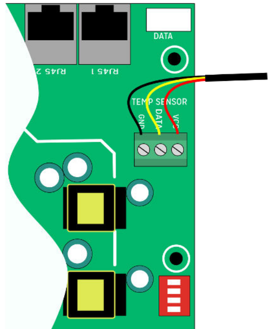
Electrical Connections
